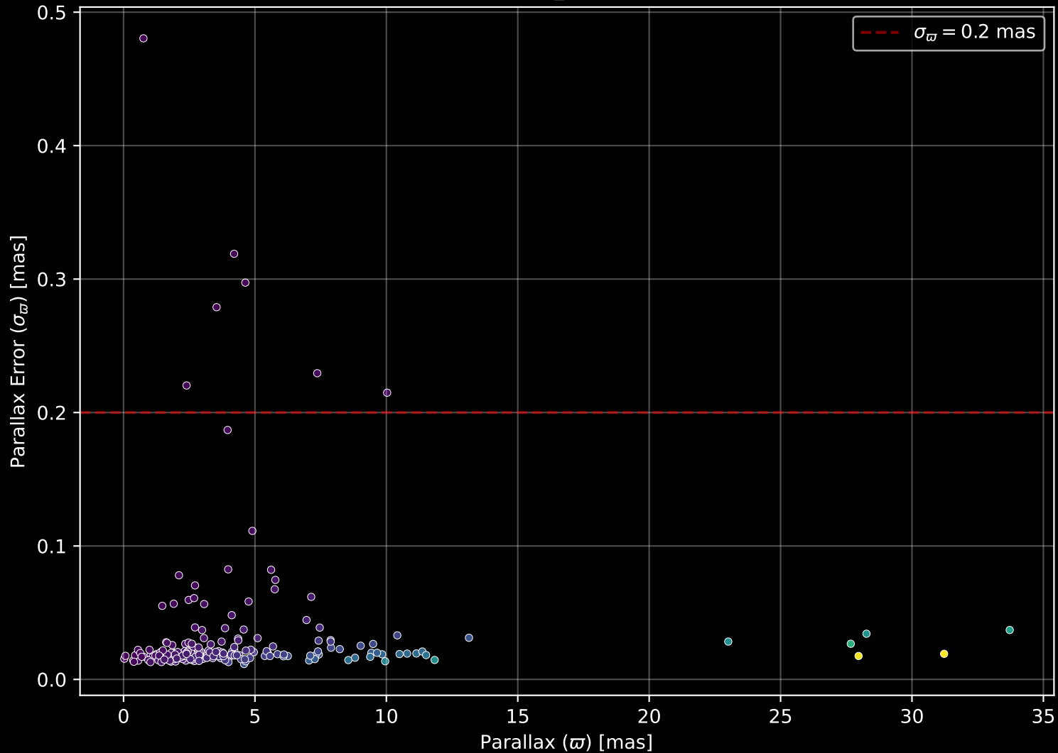
APOGEE DR17 Field: [151+70_MGA] Parallax Quality (n= 204)
