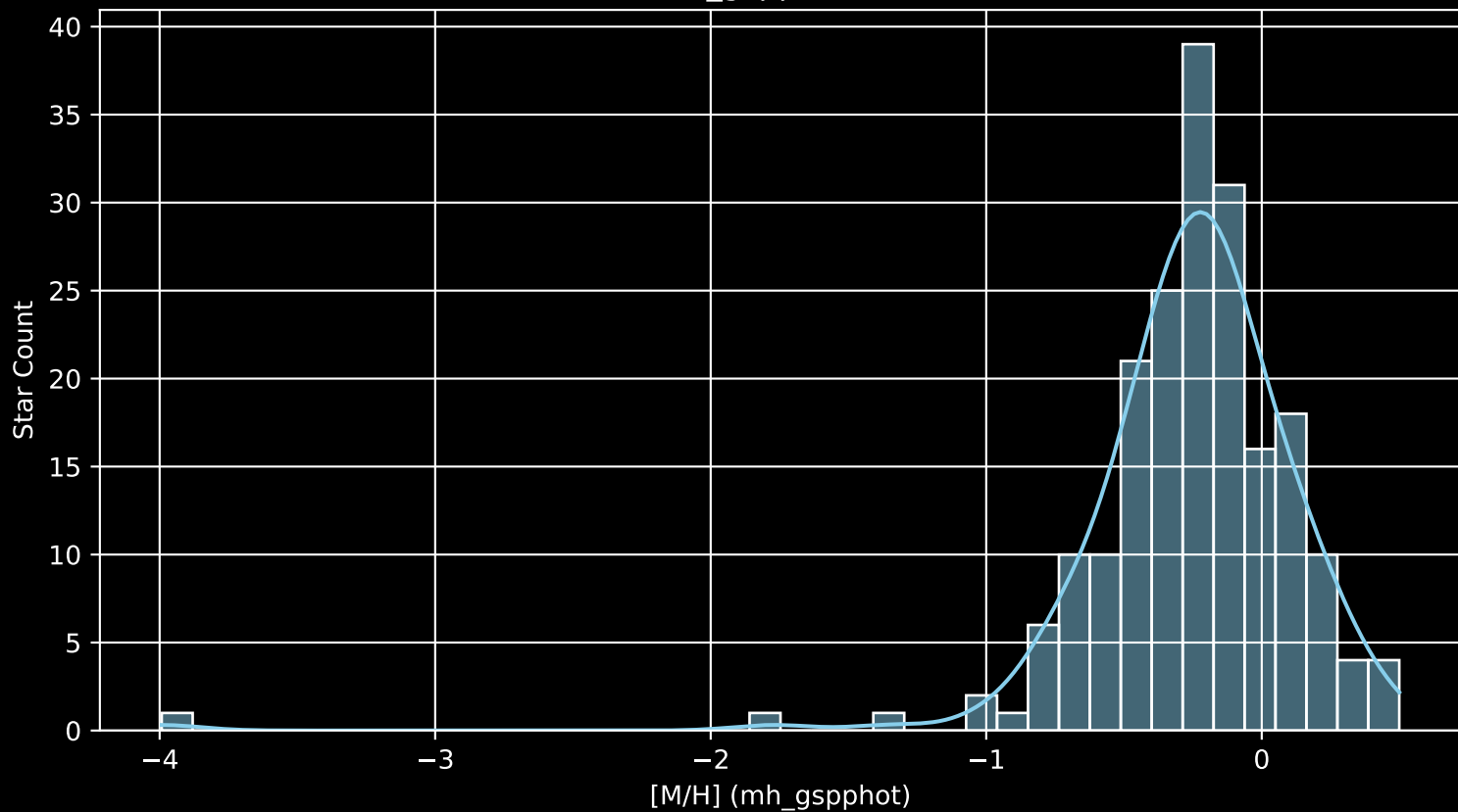
APOGEE DR17 Field: [151+70_MGA [M/H] (mh_gspphot) (n= 200)
