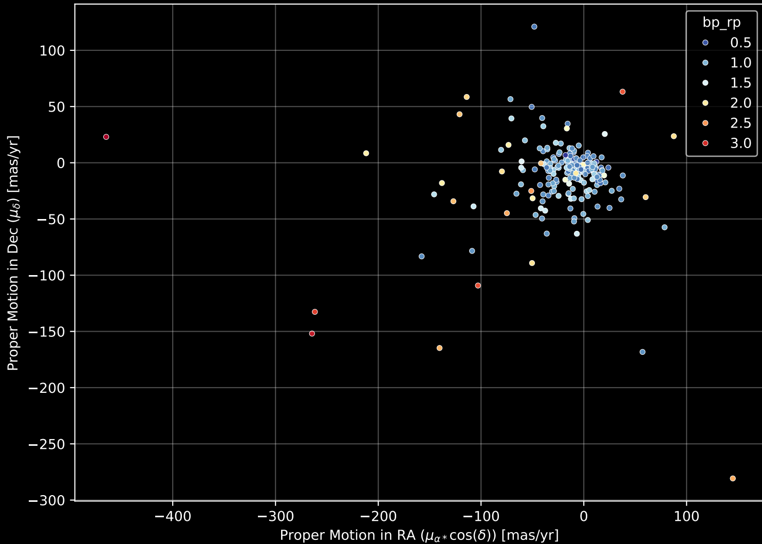
APOGEE DR17 Field: [151+70_MGA] Proper Motion Diagram (n= 204)
