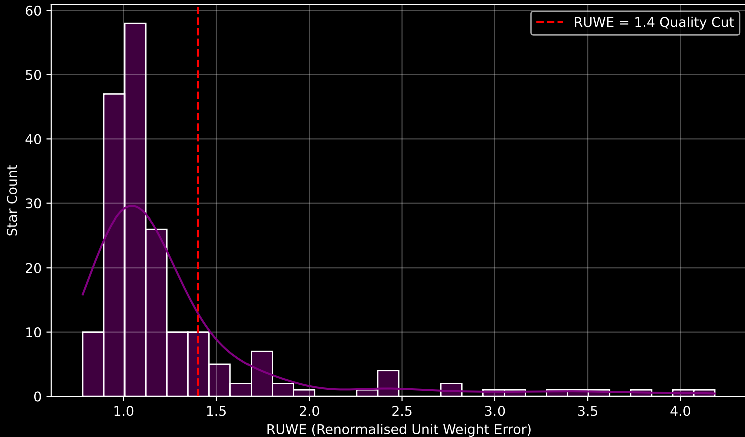
GAPOGEE DR17 Field [151+70_MGA] RUWE Distribution (n= 193)
