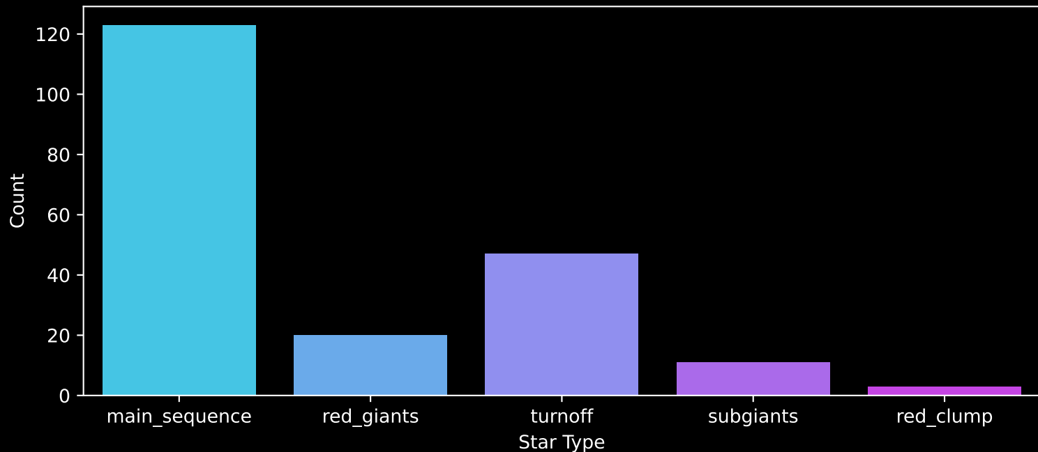
APOGEE DR17 Field: [151+70_MGA] Count plot of Star Type
